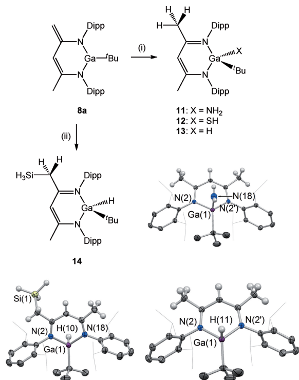
Scheme 4. Differing regioselectivities in the activation of protic and hydric H–X bonds by 8a . Key reagents and conditions: i) (for 11/12 ) excess NH 3 /H 2 S gas, benzene, RT, 30 min (decolorization in < 2 min), 60–75 %; (for 13 ) H 2 (ca. 4 atm), benzene, 70 °C, 7 h, 54 %; ii) SiH 4 (1 atm), benzene, RT, 1 h, 62 %. Molecular structures of 11 (upper), 13 (lower right) and 14 (lower left) determined by X-ray crystallography (see Supporting Information for 12 ). Most H atoms omitted, and selected C atoms shown in wireframe format for clarity; thermal ellipsoids at 50 % probability level.
